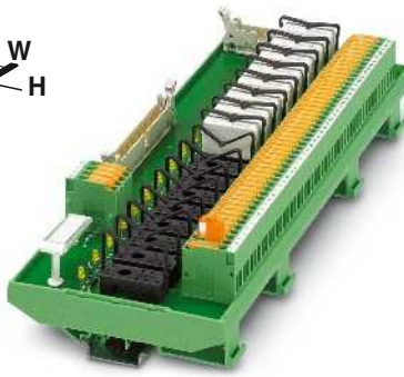
Output module for 16 miniature relays with knife/disconnect terminal blocks, 1 PDT
