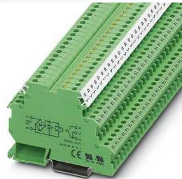
for small to medium loads 1 N/O contact (1)
