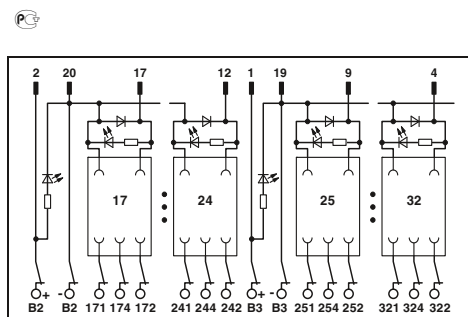
Output extension module for 16 miniature relays with knife/disconnect terminal blocks, 1 PDT
