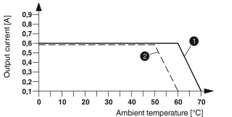
Derating curve ELR H3-IES-SC-230AC/500AC-0,6 100% operating time
