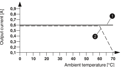
Derating curve ELR H3-IES-SC-24DC/500AC-0,6 100% operating time
