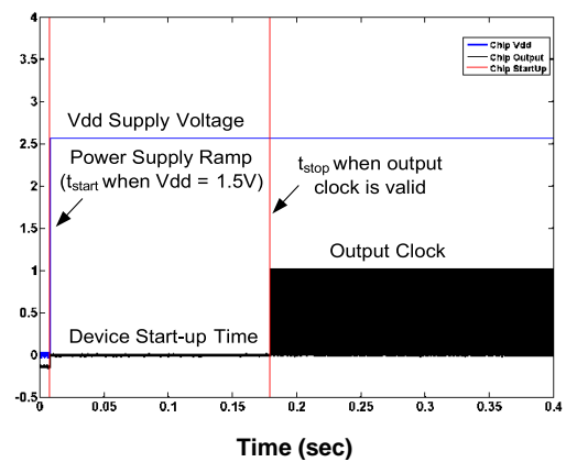
Figure 8. Start-up Time
