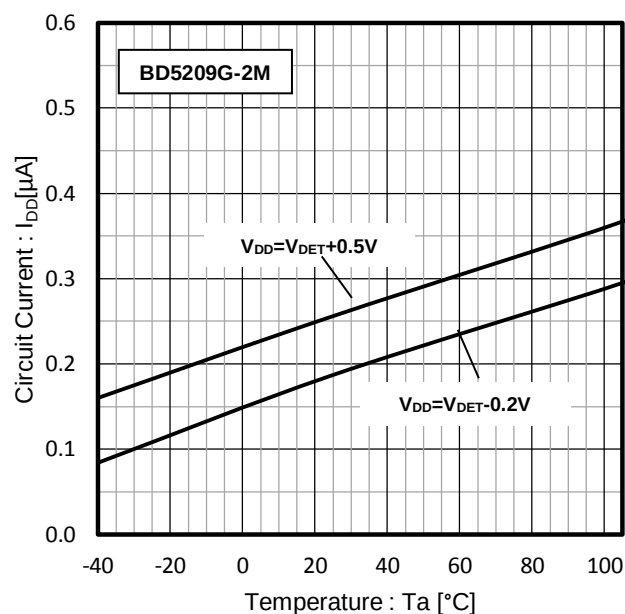
Figure 6. Circuit Current vs. Temp
