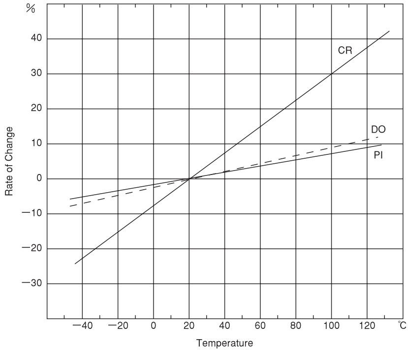
(1) Temperature Characteristics
