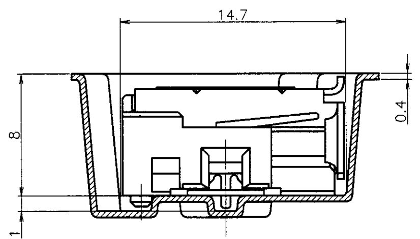
DETAIL "A" (SCALE 4-1)
