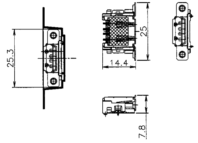
CONNECTOR DETAIL
