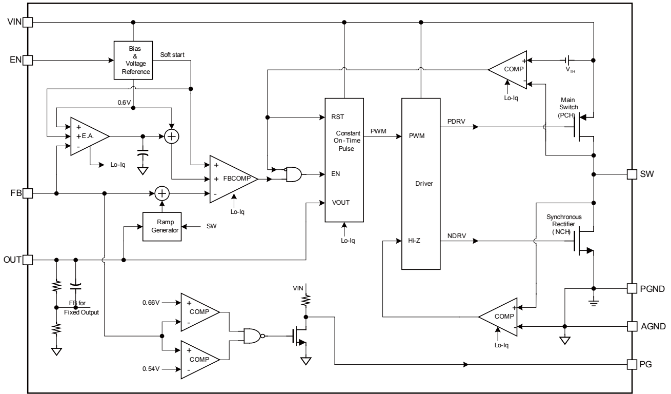
Figure 1: MP2161A Block Diagram
