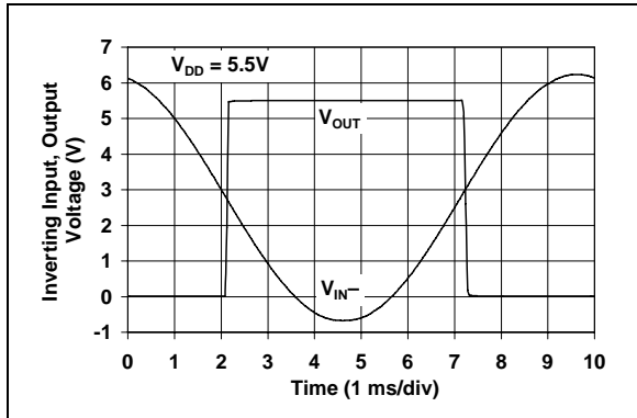
FIGURE 2-3: The MCP6546/6R/6U/7/8/9 Comparators Show No Phase Reversal.
