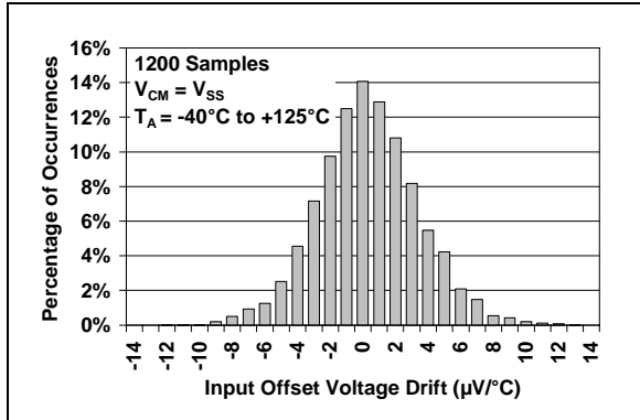
FIGURE 2-2: Input Offset Voltage Drift at V_{CM} = V_{SS} .
