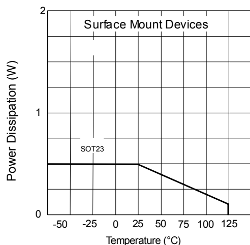
Power Derating
