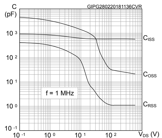
Figure 10. Capacitance variations
