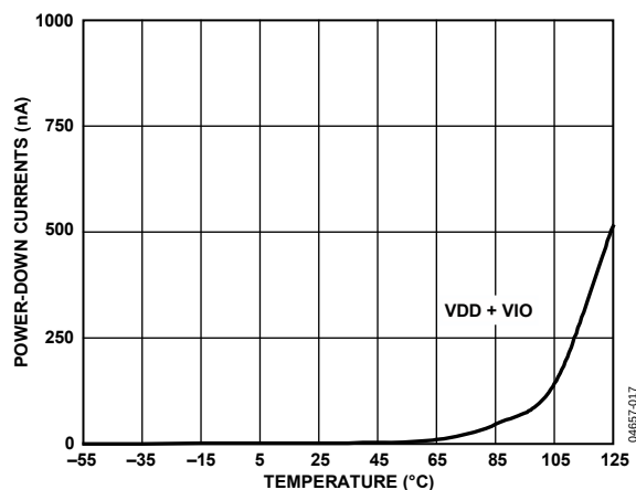
Figure 17. Power-Down Currents vs. Temperature
