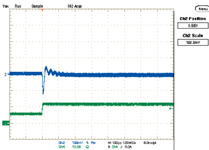
Step Load Transient Response (Vin=12V, Vout=3.3V, Load=188μF, Iout=6A to 12A) Trace 2=Vout, 100 mV/div, Trace 4=Iout, 10A/div.
