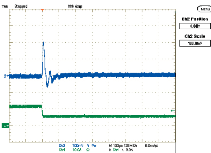
Step Load Transient Response (Vin=12V, Vout=5.0V, Cload=188uF, Iout=12A to 6A) Trace 2=Vout, 100 mV/div, Trace 4=Iout, 10A/div.
