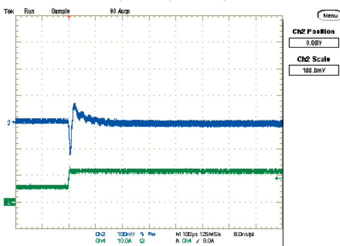
Step Load Transient Response (Vin=12V, Vout=2.5V, Cload=188μF, Iout=6A to 12A) Trace 2=Vout, 100 mV/div, Trace 4=Iout, 10A/div.
