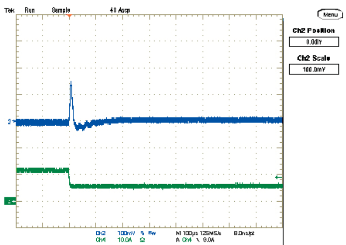
Step Load Transient Response (Vin=12V, Vout=3.3V, Load=188μF, Iout=12A to 6A) Trace 2=Vout, 100 mV/div, Trace 4=Iout, 10A/div.
