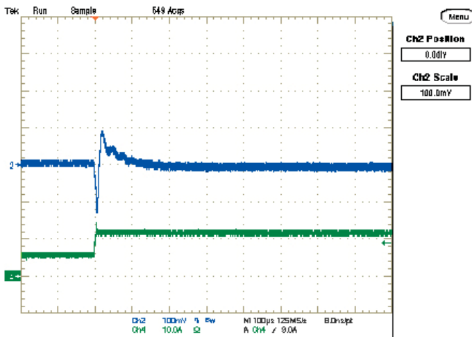
Step Load Transient Response (Vin=12V, Vout=1.8V, Cload=188μF, Iout=6A to 12A) Trace 2=Vout, 100 mV/div, Trace 4=Iout, 10A/div.
