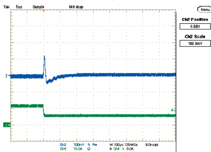
Step Load Transient Response (Vin=12V, Vout=2.5V, Cload=188μF, Iout=12A to 6A) Trace 2=Vout, 100 mV/div, Trace 4=Iout, 10A/div.
