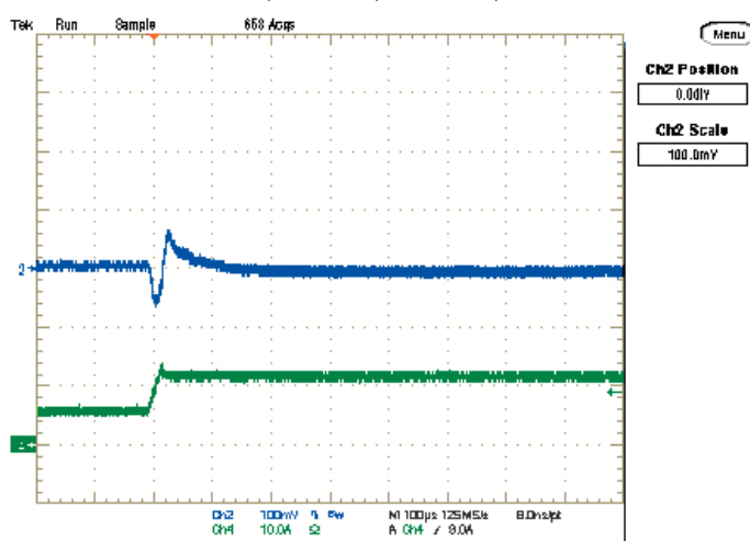
Step Load Transient Response (Vin=7V, Vout=0.69V, Cload=188μF, Iout=6A to 12A) Trace 2=Vout, 100 mV/div, Trace 4=Iout, 10A/div.
