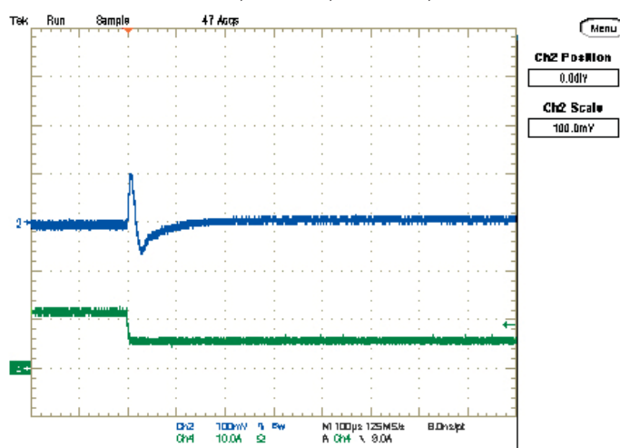
Step Load Transient Response (Vin=7V, Vout=0.69V, Cload=188μF, Iout=12A to 6A) Trace 2=Vout, 100 mV/div, Trace 4=Iout, 10A/div.
