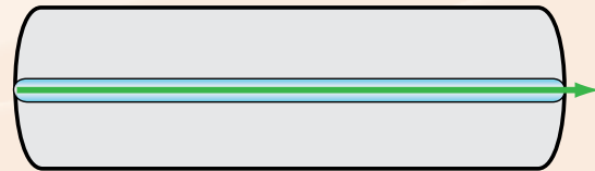
A singlemode fiber has a much thinner core than a multimode fiber. Light pulses follow a single direct path. Bandwidth essentially approaches infinity—limited practically to about 100,000 gigahertz.
