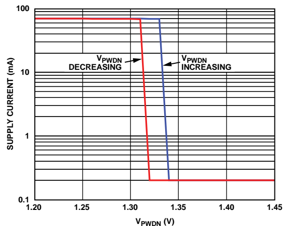
Figure 38. Supply Current vs. V_{PWDN}
