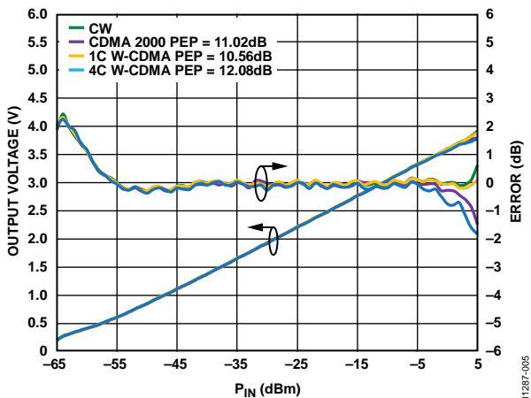
Figure 5. Error from CW Linear Reference vs. Signal Modulation (CDMA 2000, One-Carrier W-CDMA, Four-Carrier W-CDMA), Frequency = 2.14 GHz, CRMS = 0.1 \mu F, Three Point Calibration at 0 dBm, -40 dBm, and -55 dBm
