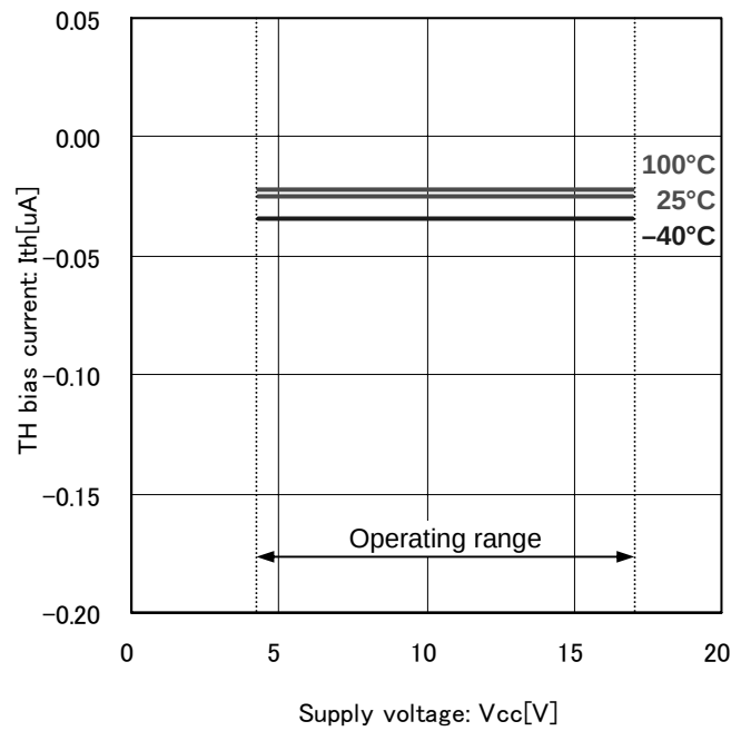
Fig.24 TH bias current
