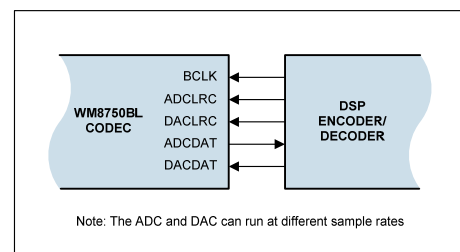
Figure 17 Slave Mode
