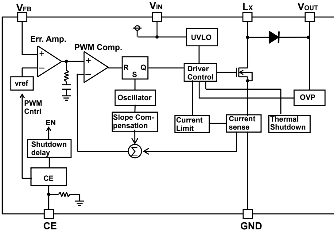
● R1205x8xxB/C
