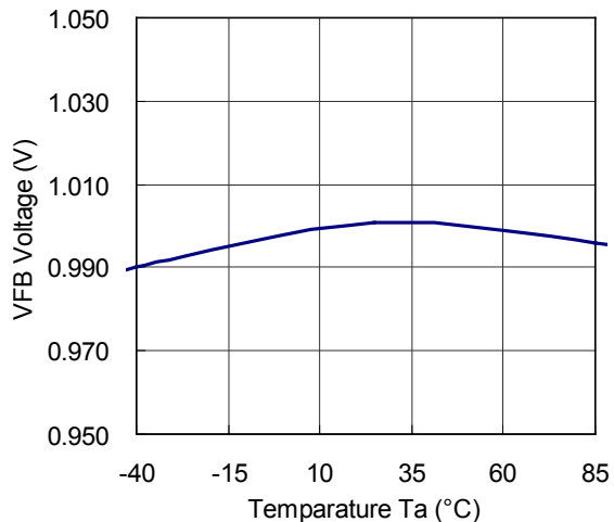
R1205x8xxA
