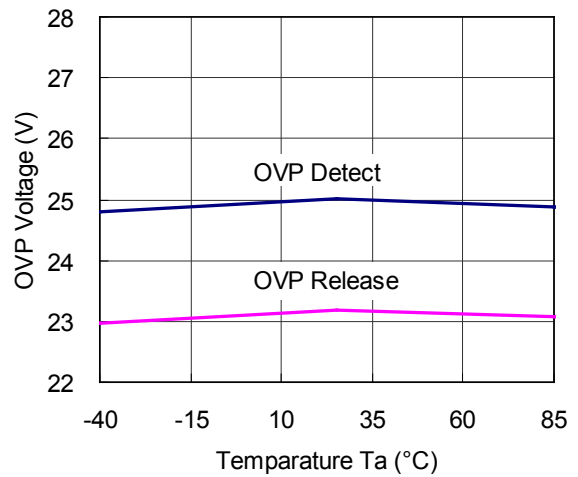
13) OVP Voltage vs. Temperature
