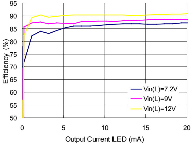
5LED, V_{IN(IC)}=3.6V
