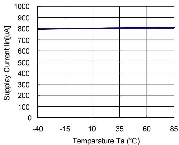
R1205x8xxB/C
