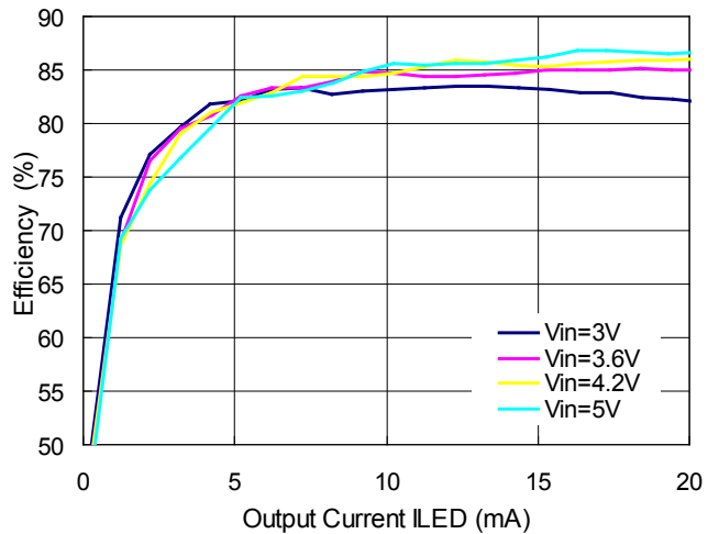
4LED, L=22\mu H (LQH32CN220K53)
