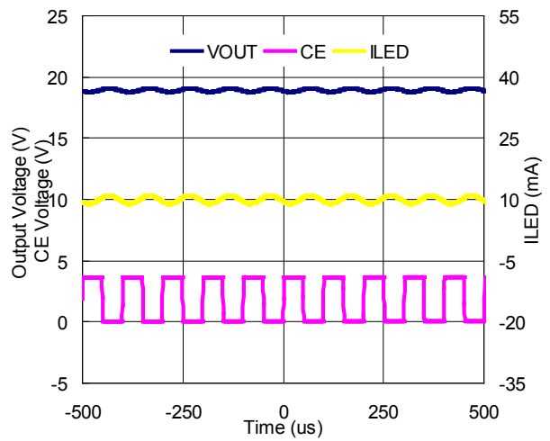
R1205N823B/C (CE Freq=10KHz)
