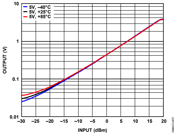
Figure 8. V_{\text{RMS}} Output vs. Input Level and Temperature at 1900\text{ MHz} , Supply 5V
