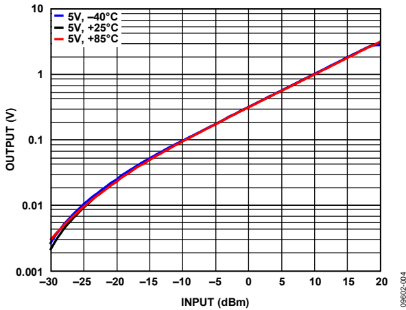
Figure 5. V_{\text{ENV}} - V_{\text{REF}} Output vs. Input Level and Temperature at 1900\text{ MHz} , Supply 5V
