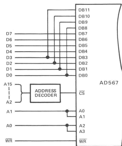
Right-justified data can be similarly accommodated. The overlapping of data lines is reversed, and the address connections are slightly different. The AD567 still occupies two adjacent locations in the processor's memory map.
