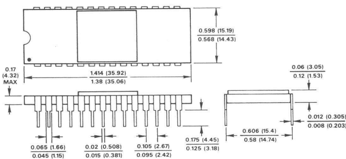
28-Pin Ceramic DIP (D Package)
