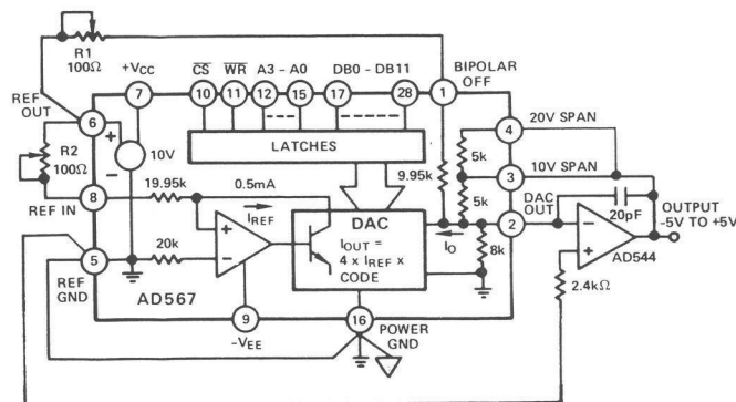
Figure 2. \pm 5V Bipolar Voltage Output
