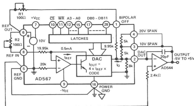
Figure 2. \pm 5\text{V} Bipolar Voltage Output
