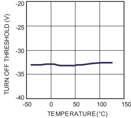
Turn off threshold vs. Temperature
