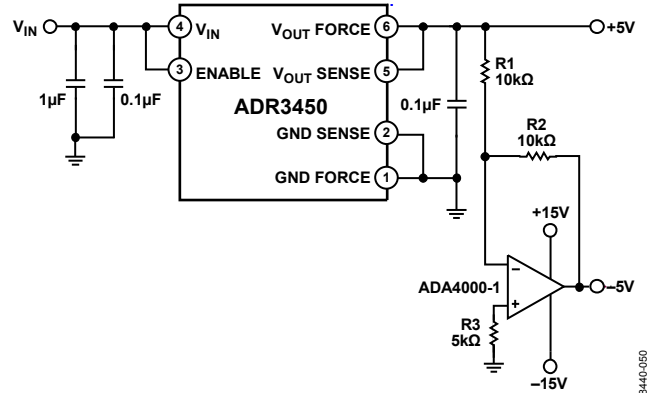
Figure 43. ADR3450 Bipolar Output Reference
