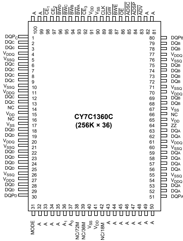
Figure 1. 100-pin TQFP (14 x 20 x 1.4 mm) pinout (3 Chip Enables - A Version)
