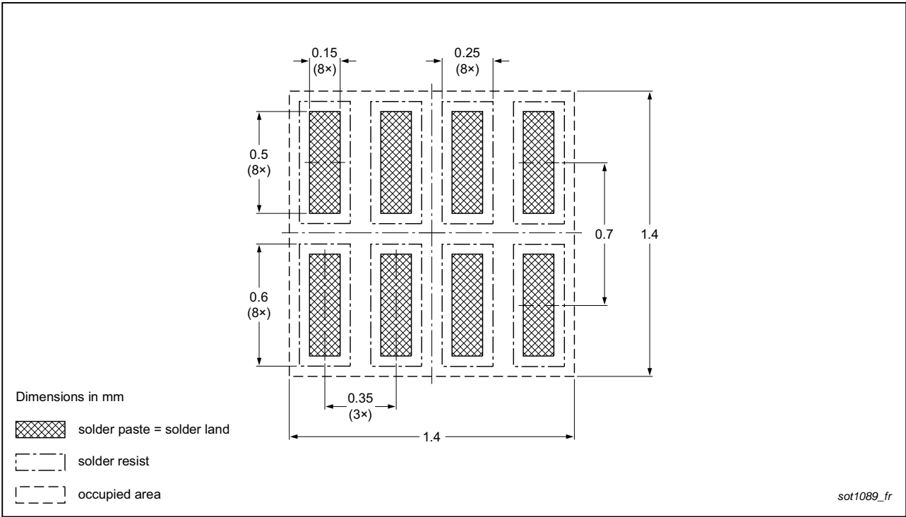
Fig 27. PCB footprint for SOT1089 (XSON8); reflow soldering
