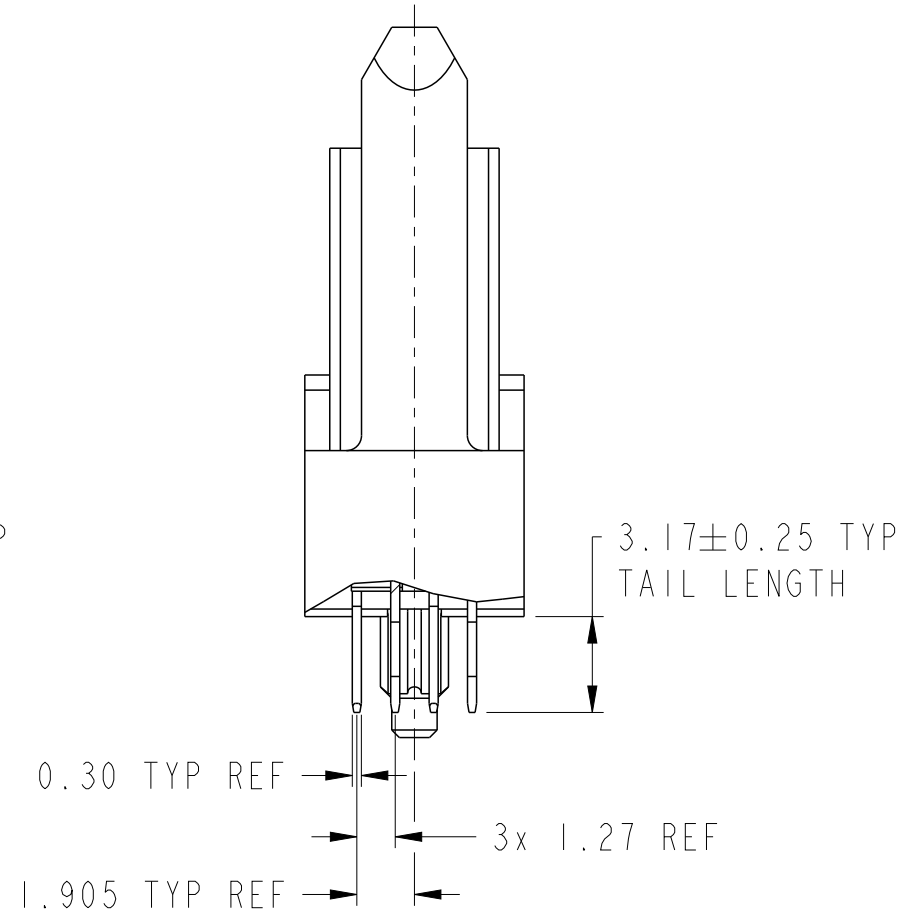
SECTION B-B
