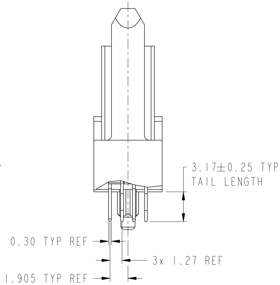
SECTION B-B
