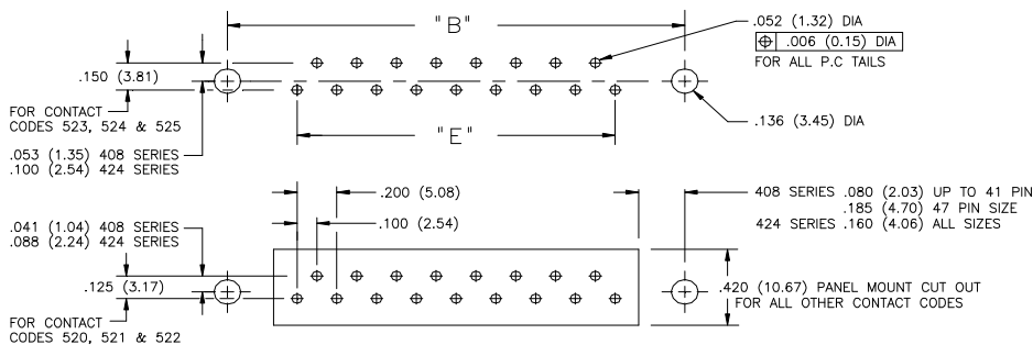
CONNECTOR MOUNTING PATTERNS FOR 408 & 424 SERIES
