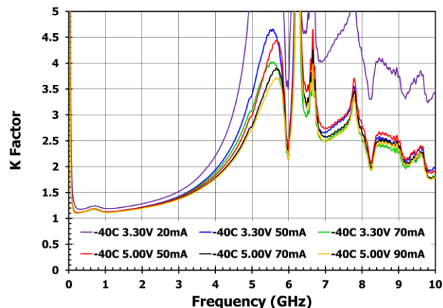
Figure 32. Stability Factor for Various Currents (3.3V, 5.0V, -40°C, R8=1K)
