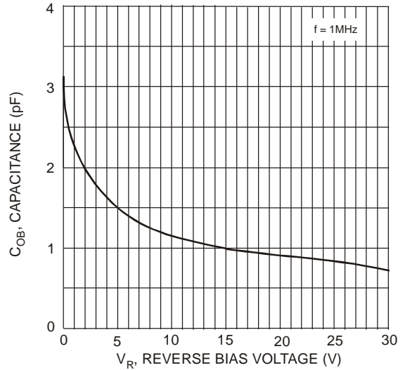
Fig. 4 Output Capacitance
