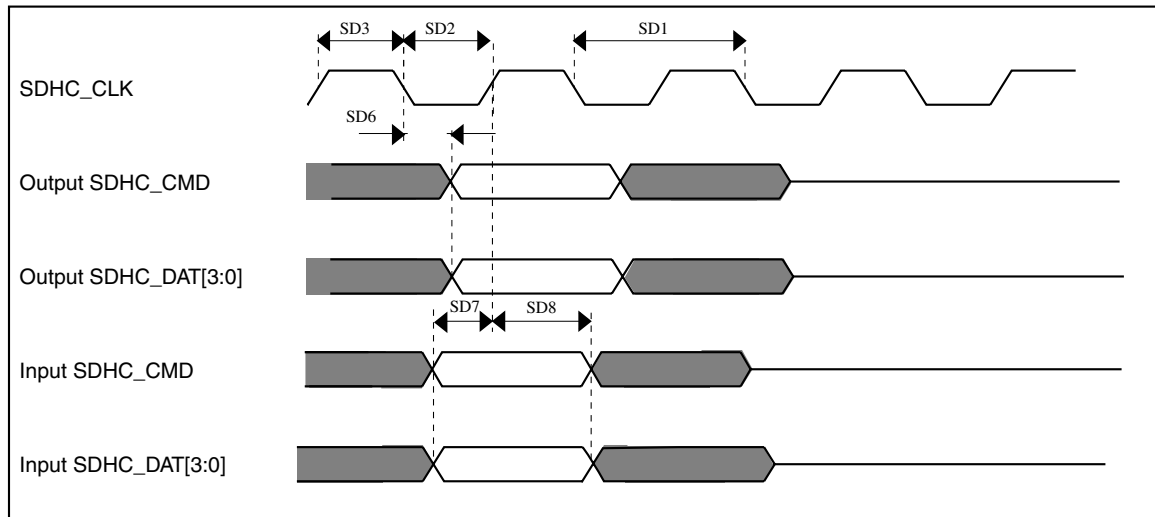
Figure 32. SDHC timing
