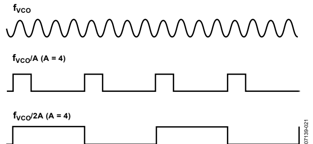
Figure 21. DIVOUT Waveforms
