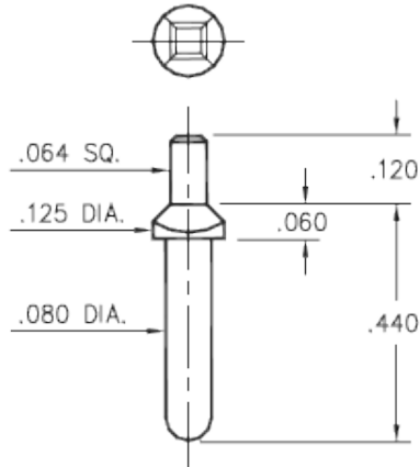
8952-0-05-XX-00-00-03-0 Square press-fit in .087 plated thru hole
