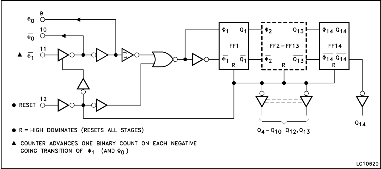
Figure 2. Logic diagram
