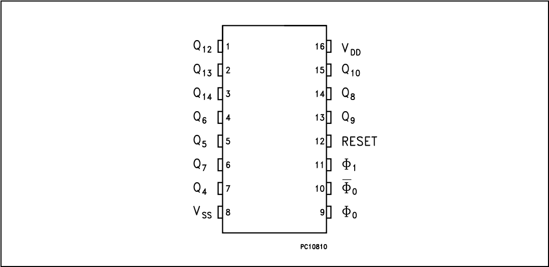
Figure 1. Pin connection
