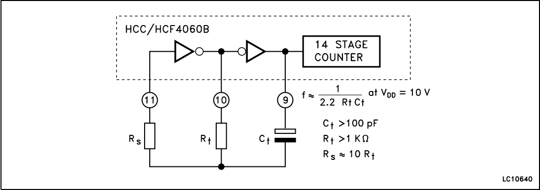
Figure 6. Typical RC oscillator circuit
