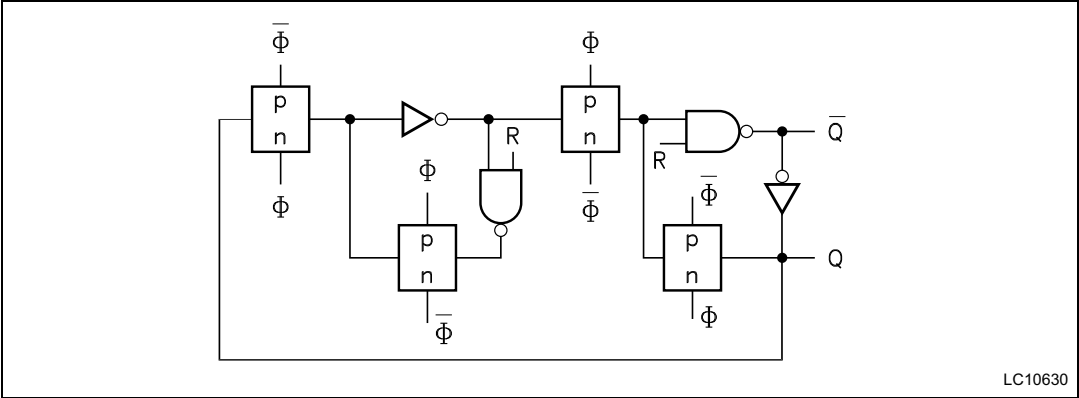
Figure 5. Detail of typical flip-flop stage
