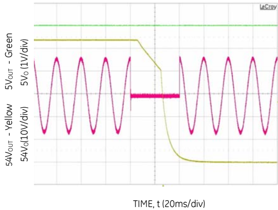
Figure 13. 40ms AC dropout @ full load, V IN = 230V AC .
