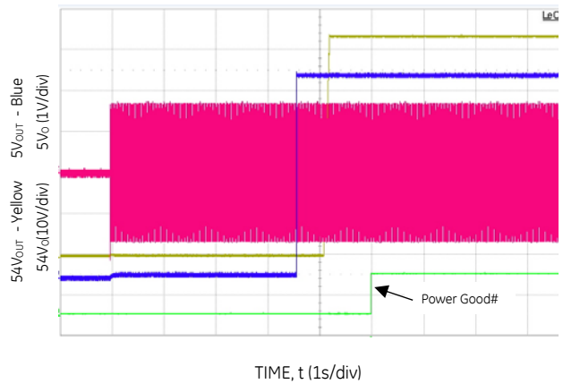
Figure 14. Turn-ON at full load V IN = 230V AC .
