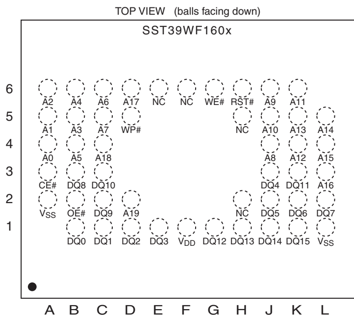
FIGURE 2: Pin assignments for 48-ball WFBGA
