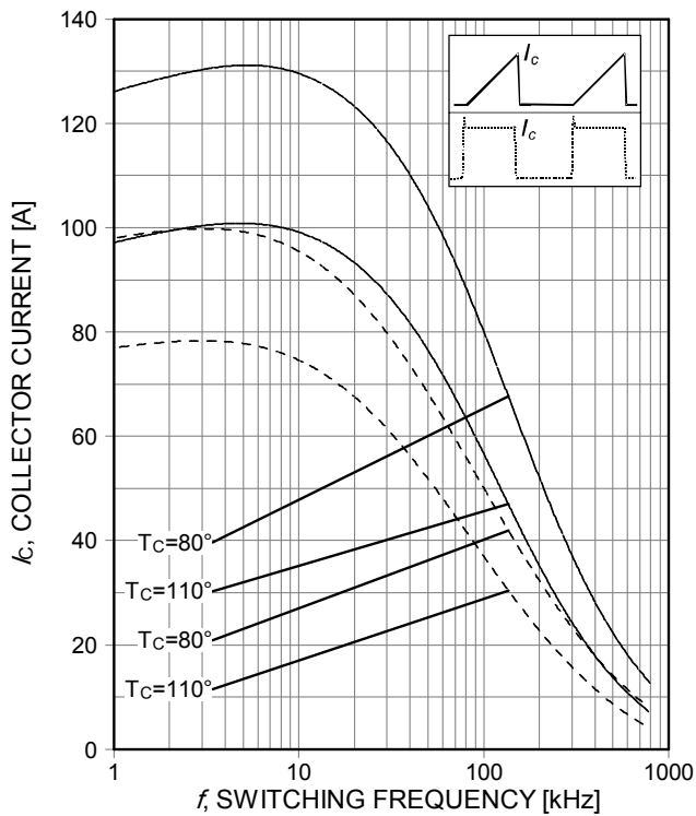
Figure 1. Collector current as a function of switching frequency ( T_j \leq 175^\circ\text{C} , D=0.5 , V_{CE}=400\text{V} , V_{GE}=15\text{V} , R_G=7\Omega )
