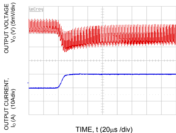
Fig-48. Transient Response to Dynamic Load Change from 50% to 100% at 12Vin, C_{out}= 1x47\mu F+11x330\mu F , C_{Tune}=47nF , R_{Tune}=178ohms
