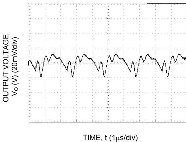
Fig-41. Typical output ripple and noise (CO=2x47µF ceramic, VIN = 12V, Io = Io,max, ).
