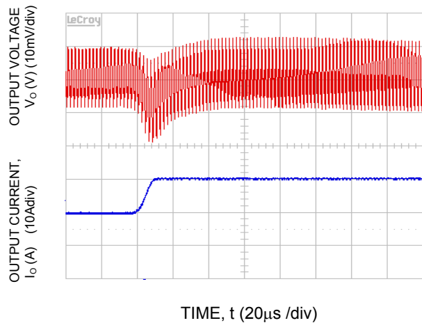
Fig-42. Transient Response to Dynamic Load Change from 50% to 100% at 12Vin, Cout= 1x47µF+5x330µF, CTune=10nF & RTune=178ohms
