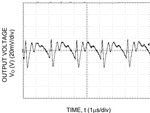
Fig-47. Typical output ripple and noise ( C_O=2x47\mu F ceramic, V_{IN} = 12V , I_o = I_{o,max} ).
