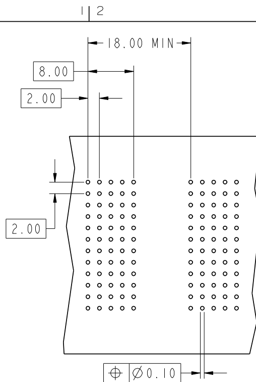
REQUIRED PC BOARD LAYOUT COMPONENT SIDE SEE PRINT 58351 FOR ADDITIONAL PCB INFORMATION
