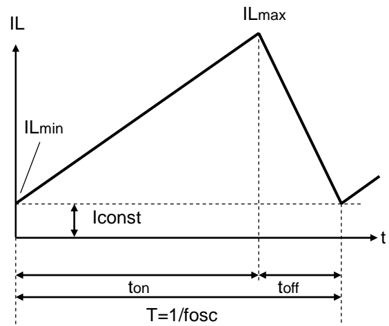
Figure 6. Continuous Mode
