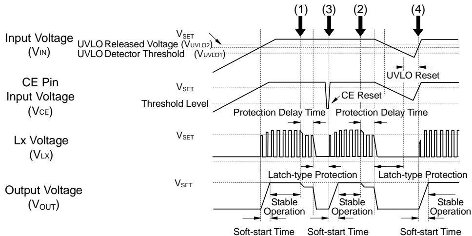
Figure 13. Timing Chart
