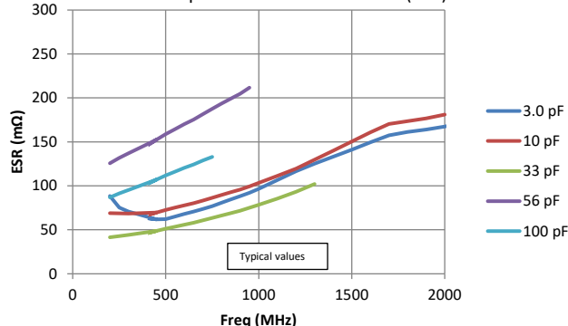
0201 R05L Equivalent Series Resistance (ESR)
