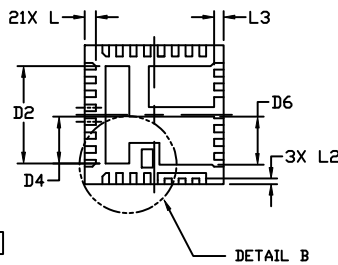
SUPPLEMENTAL BOTTOM VIEW
