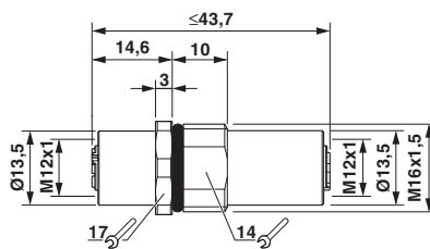
Dimensioned drawing
