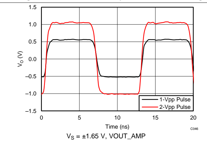
Figure 46. Pulse Response for Various V_O
