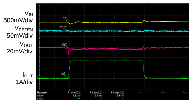
Source Load Transient (DDR-IV) ( C_{IN}=C_{OUT}=10\mu F , I_{OUT}=0A to 1.75A , V_{IN}=1.2V , V_{REFEN}=0.6V , V_{CNTL}=3.3V )
