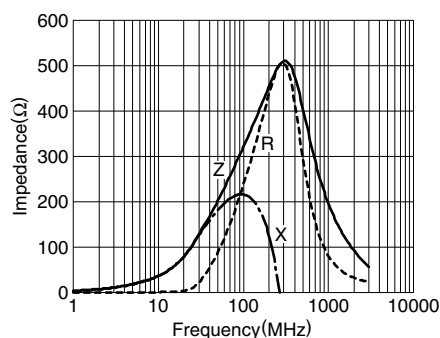
TYPICAL ELECTRICAL CHARACTERISTICS Z, X, R vs. FREQUENCY CHARACTERISTICS MMZ2012Y301B
